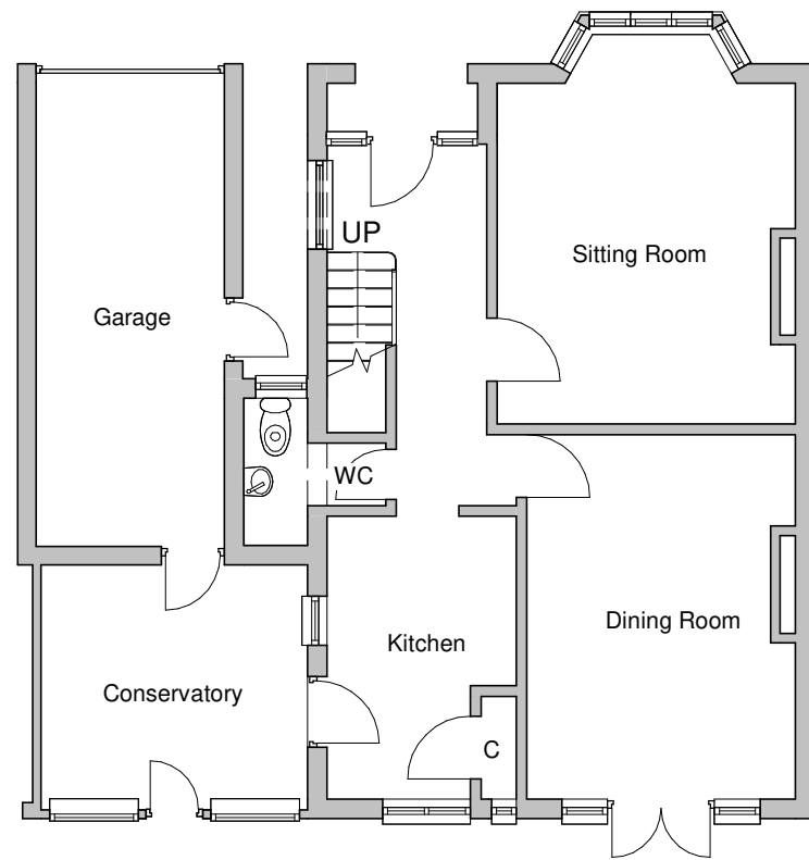
1 Ground floor 1 : 100
