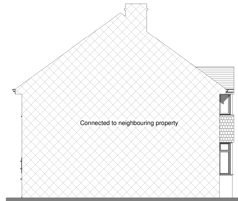
4 Existing Side 2 Elevation 1 : 100
