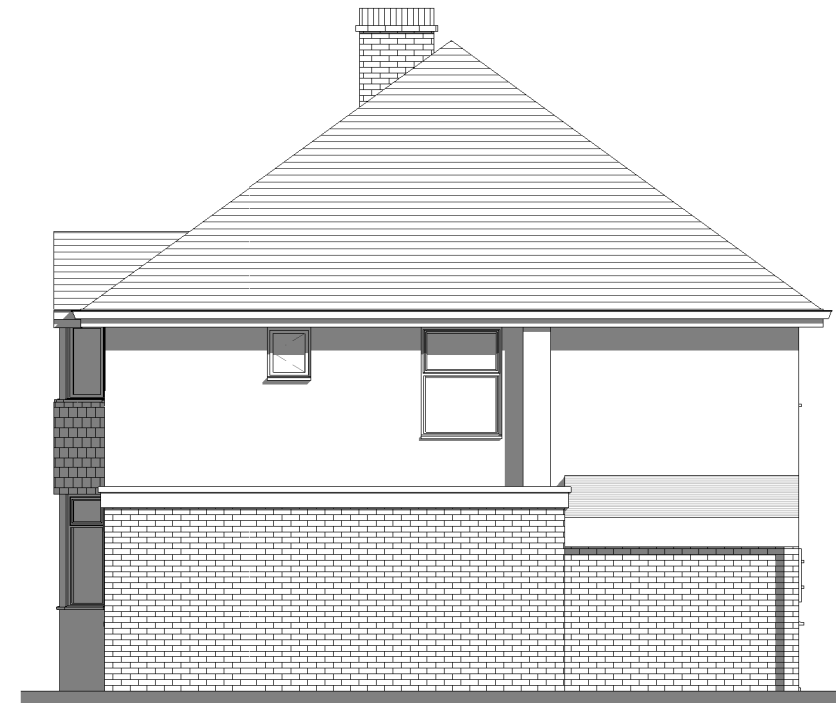
2 Existing Side 1 Elevation 1 : 100
